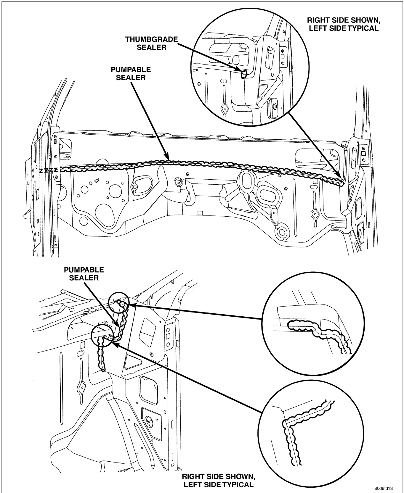
Fig. 12 DASH PANEL
